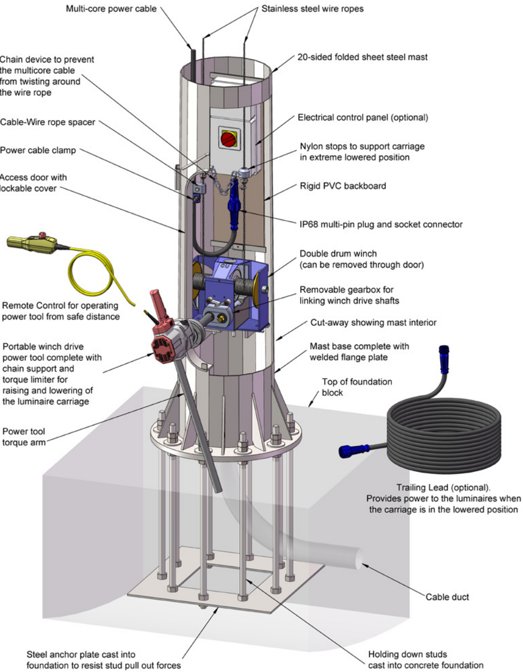
High Mast Base Arrangement (Double drum winch system shown)
